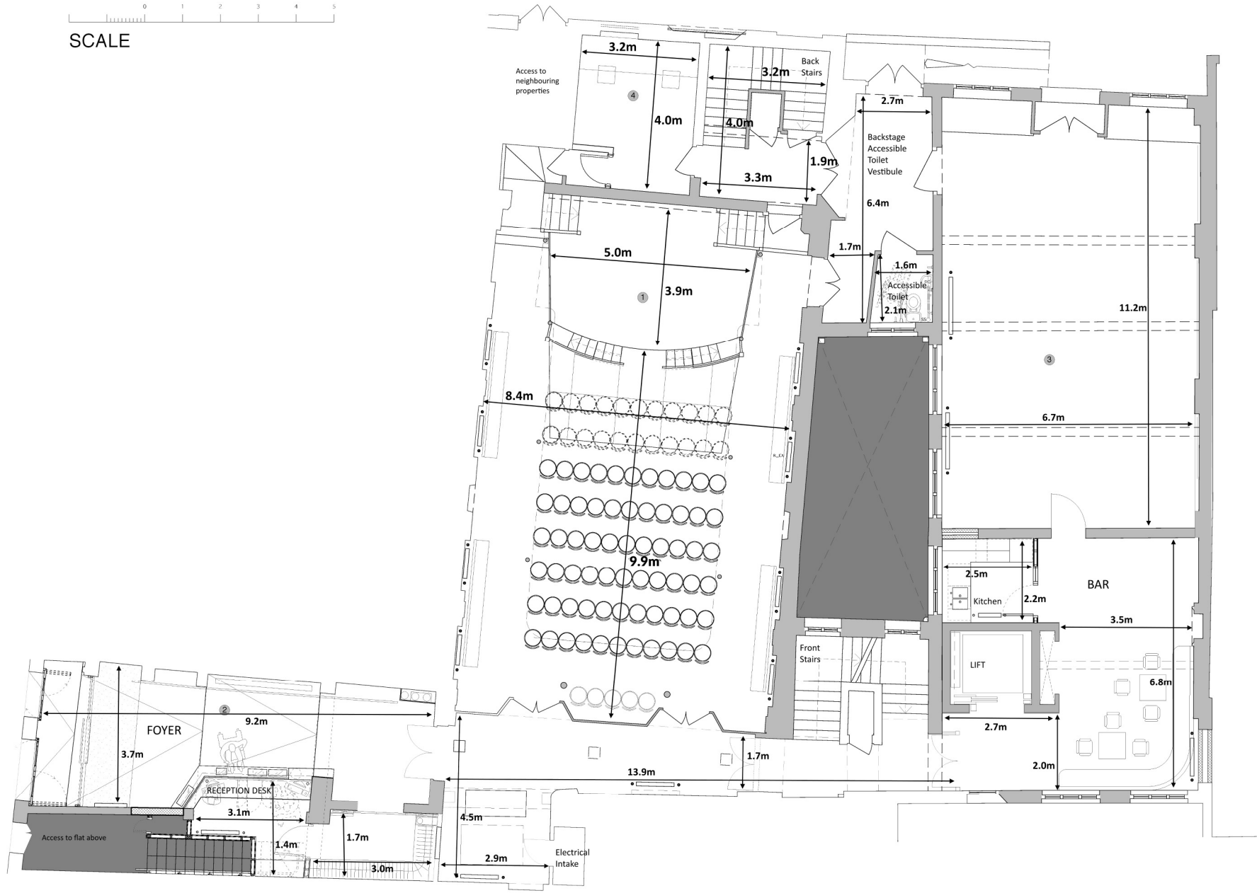
HOXTON HALL - GROUND FLOOR PLAN 1: 50 @A1
